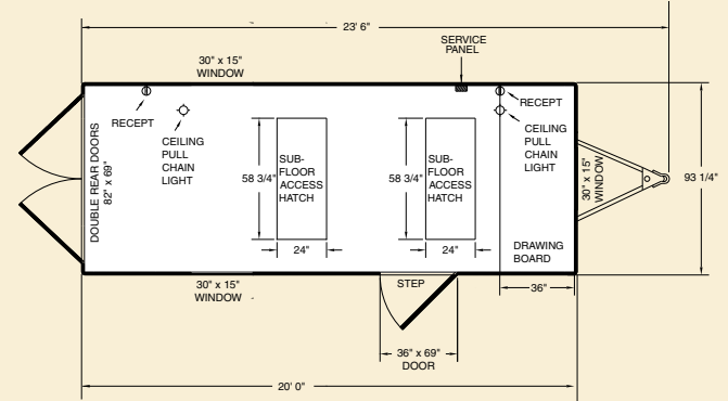
Model WW2011 & WW2022
