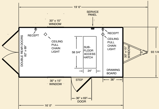
Model WW1611 & WW1622
