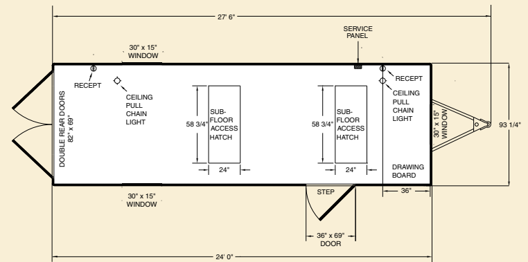
Model WW2411 & WW2422
