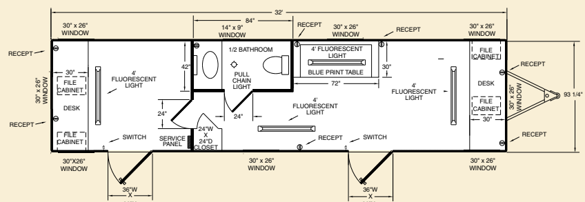
Model FO3222 with optional 1/2 Bath
